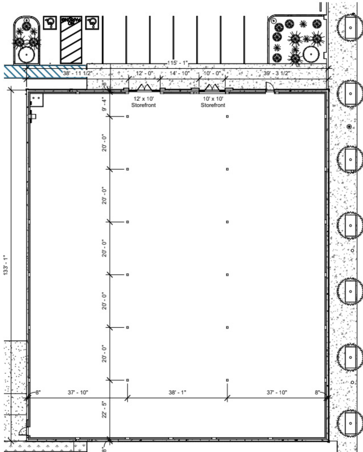
① Building Layout 1/16" = 1'-0"
